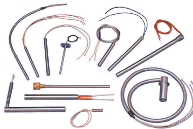
Cartridge Heaters
