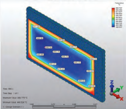
FEA ANALYSIS
