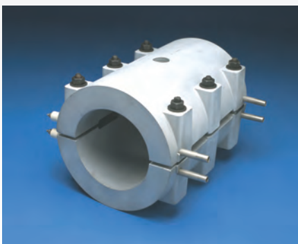
LIQUID-COOLED BARRELS
