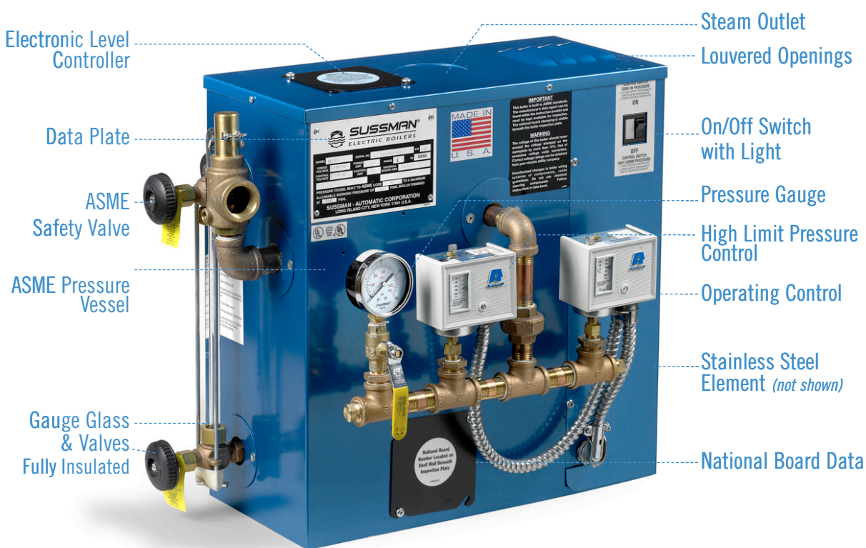
Typical boiler arrangement
